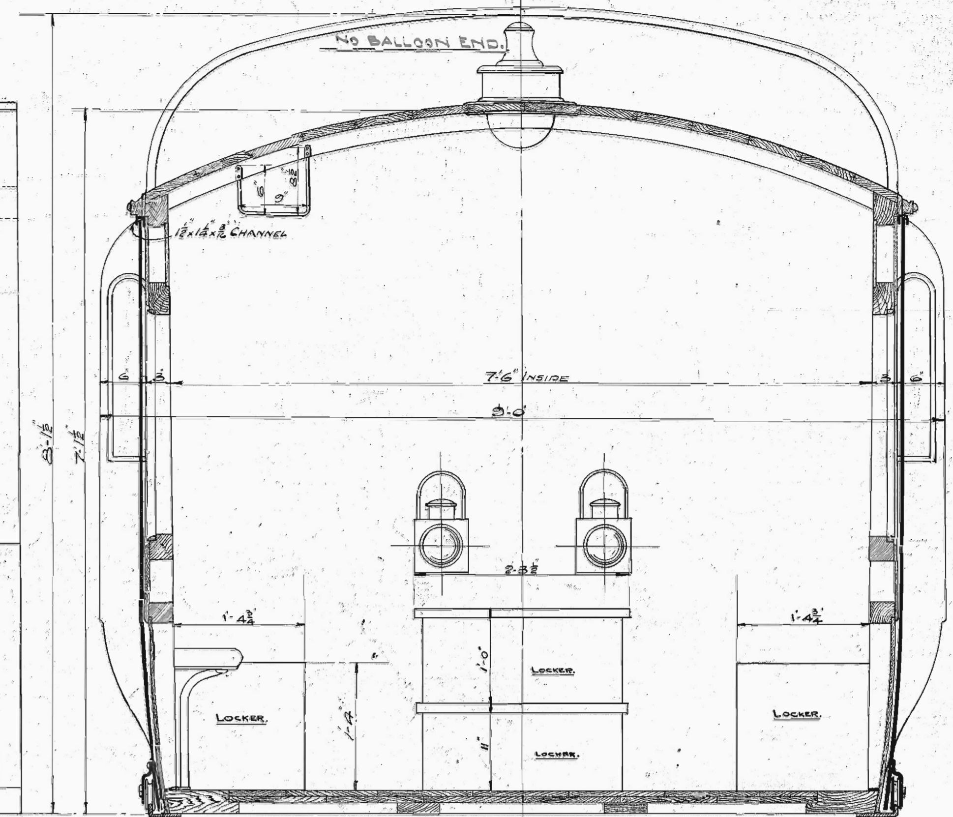
SECTION ON LINE A-B.
