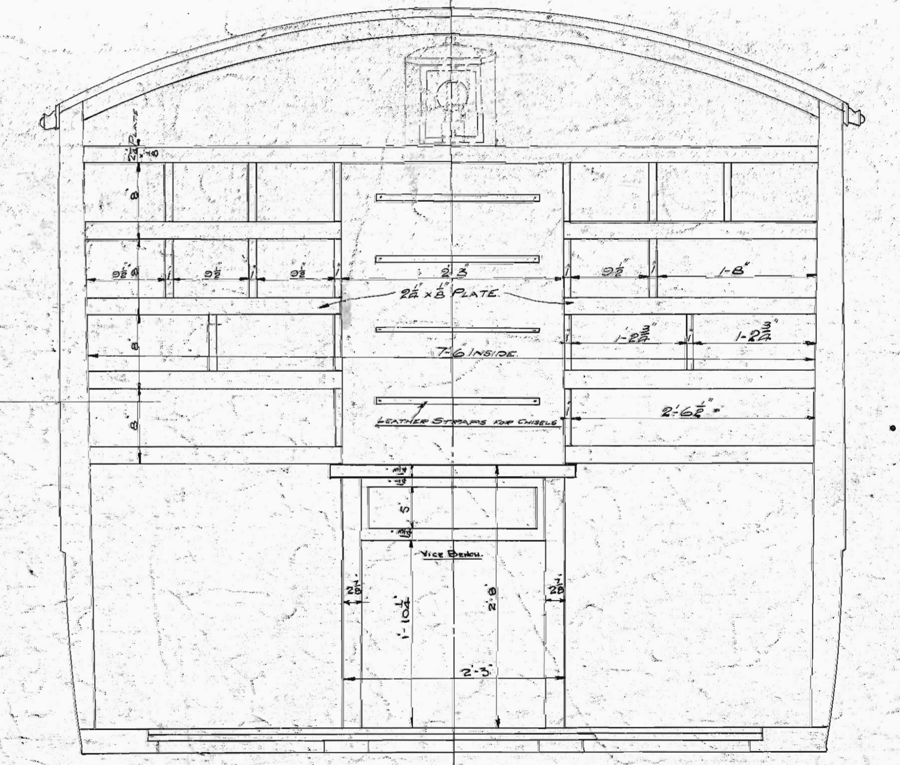
SECTION ON LINE C-D
