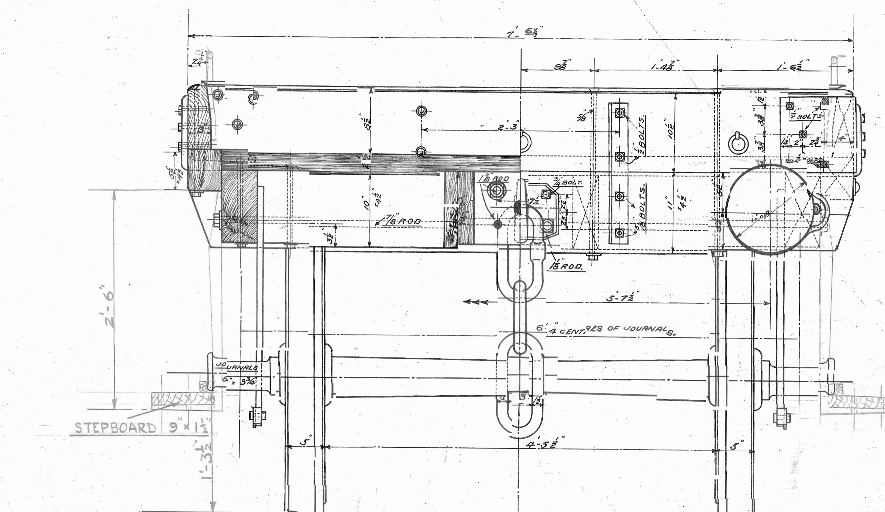
CROSS SECTION—END ELEVATION.
