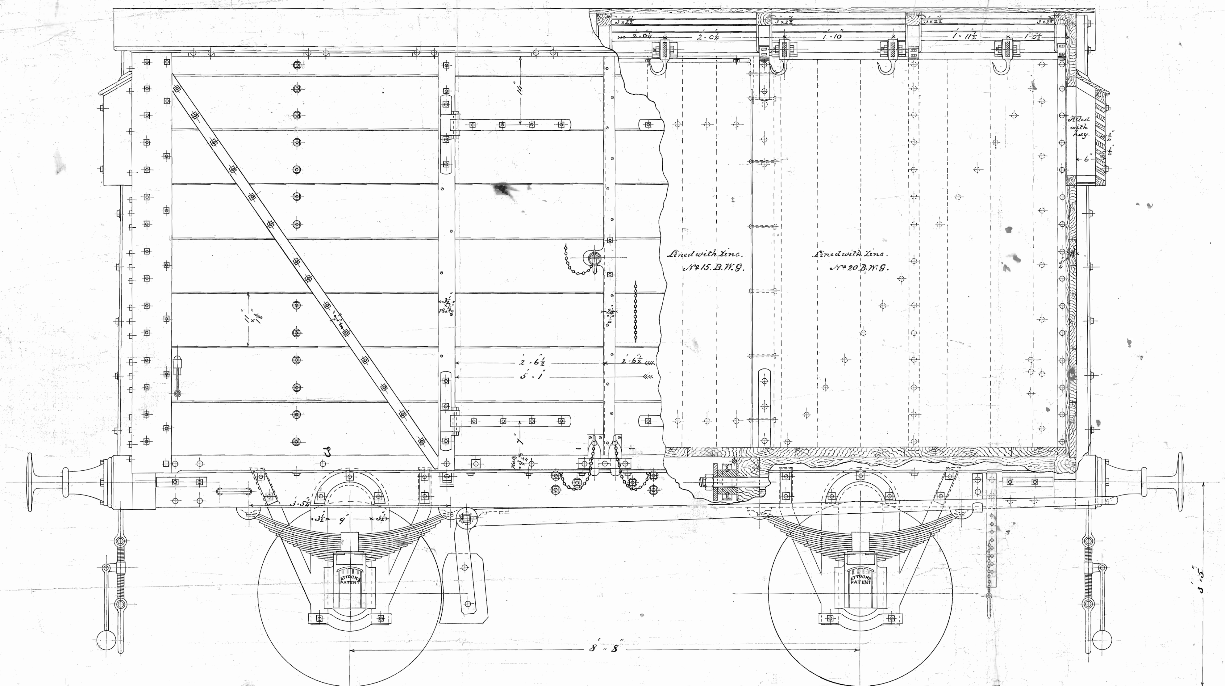
Half Side Elevation.
