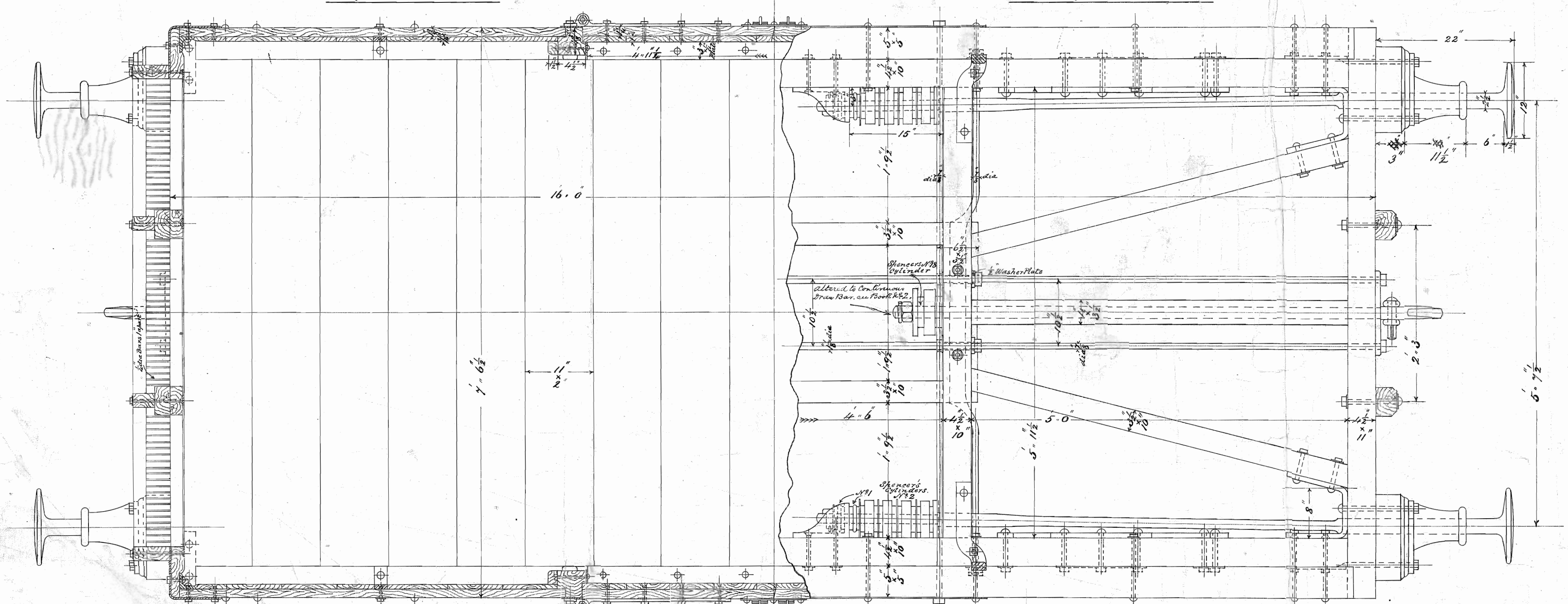
Half Sectional Plan of Body.
