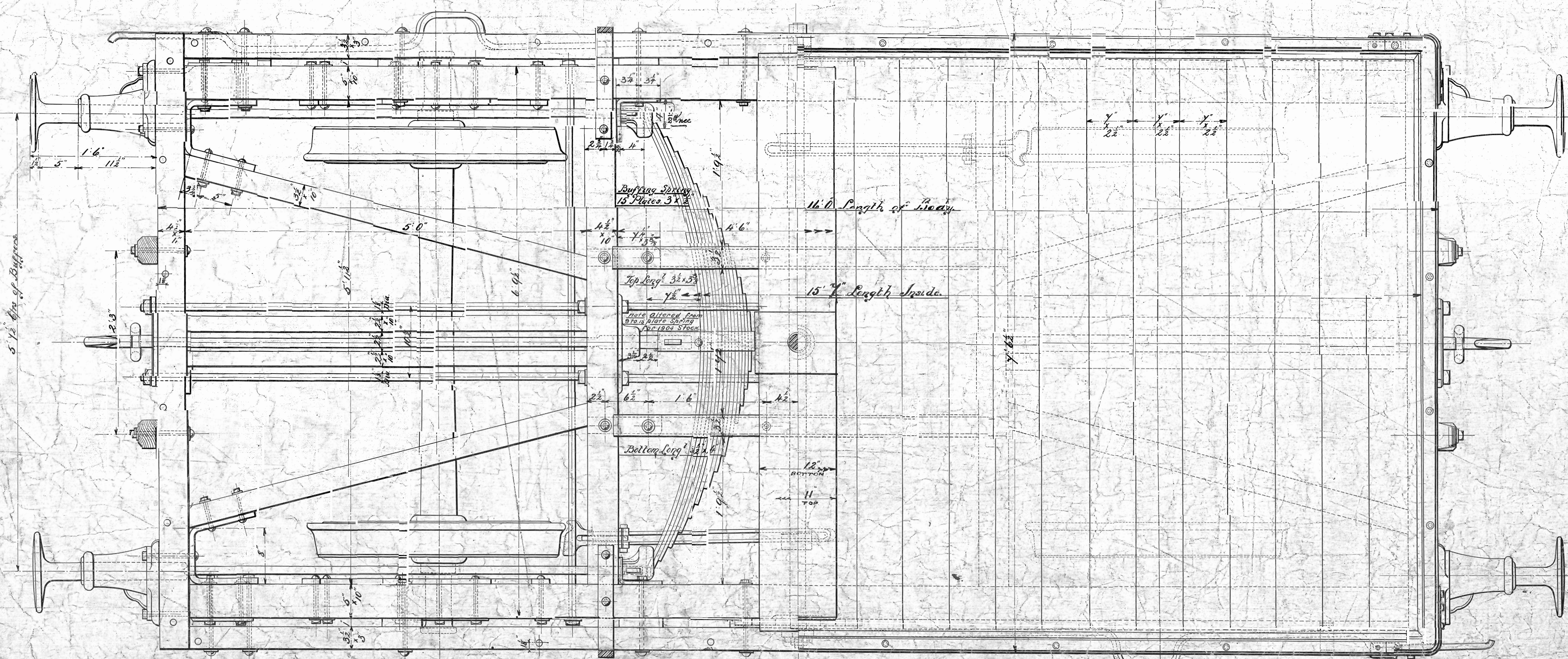
Half Plan of Underframe
