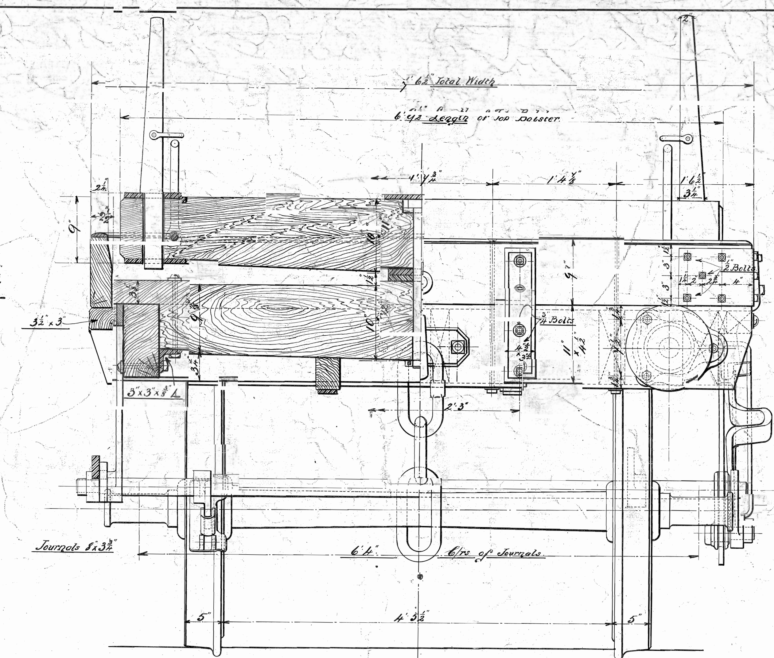
Cross Section at Center
