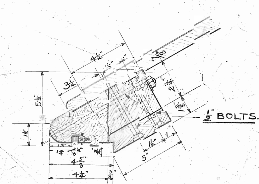
SECTION OF CANTRAIL OVER DOOR SCALE 3" TO A FOOT.
