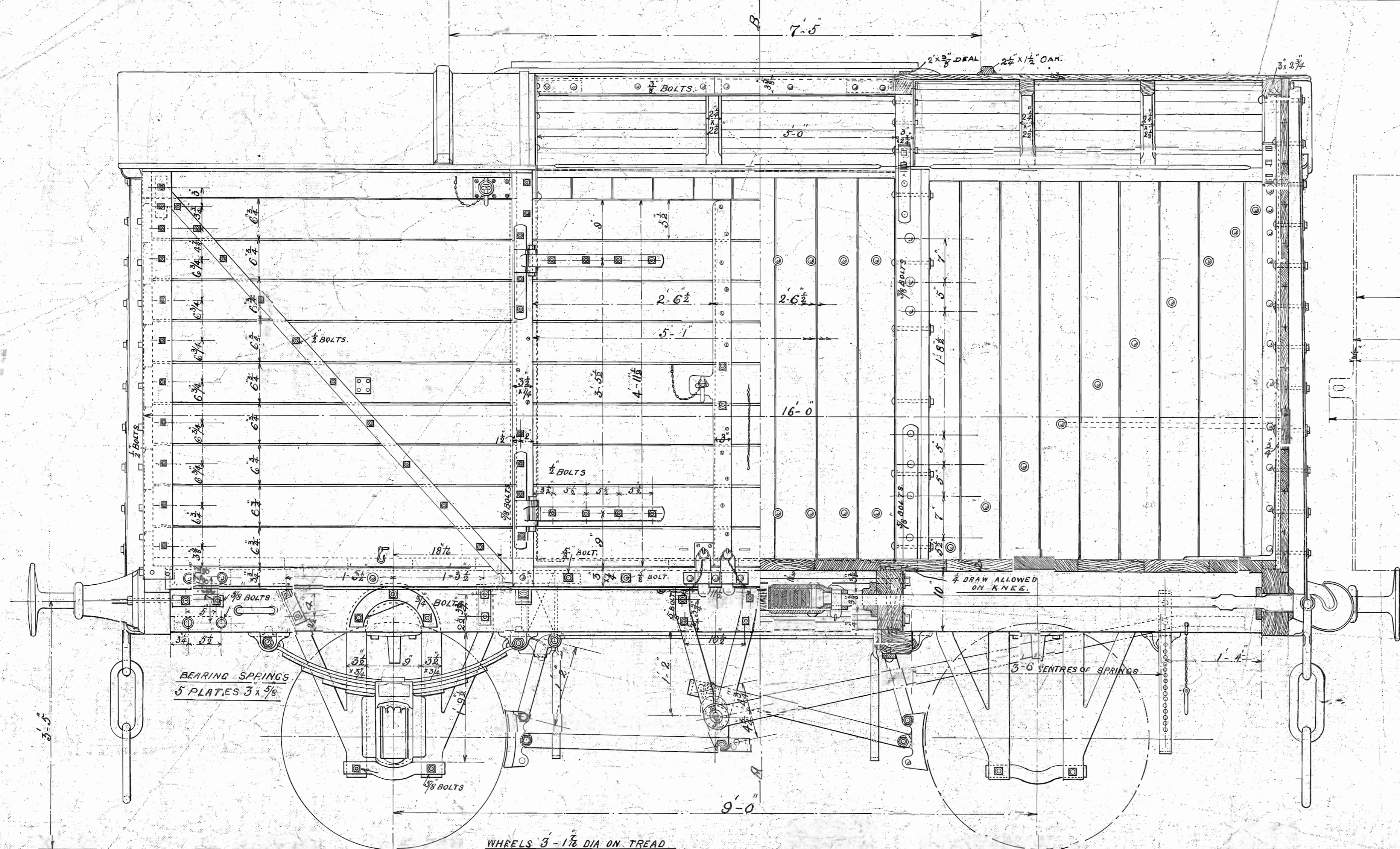
HALFSIDE ELEVATION
