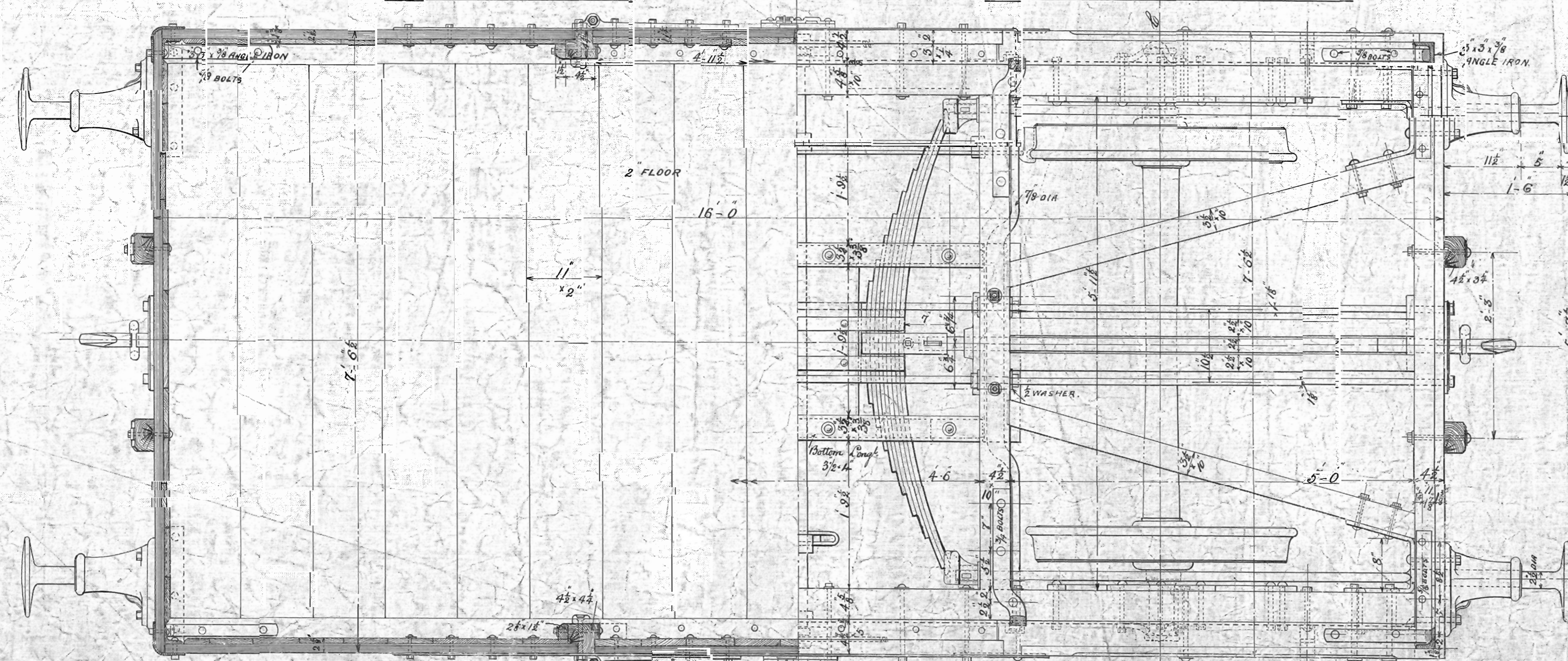
HALF SECTIONAL PLAN OF BODY
