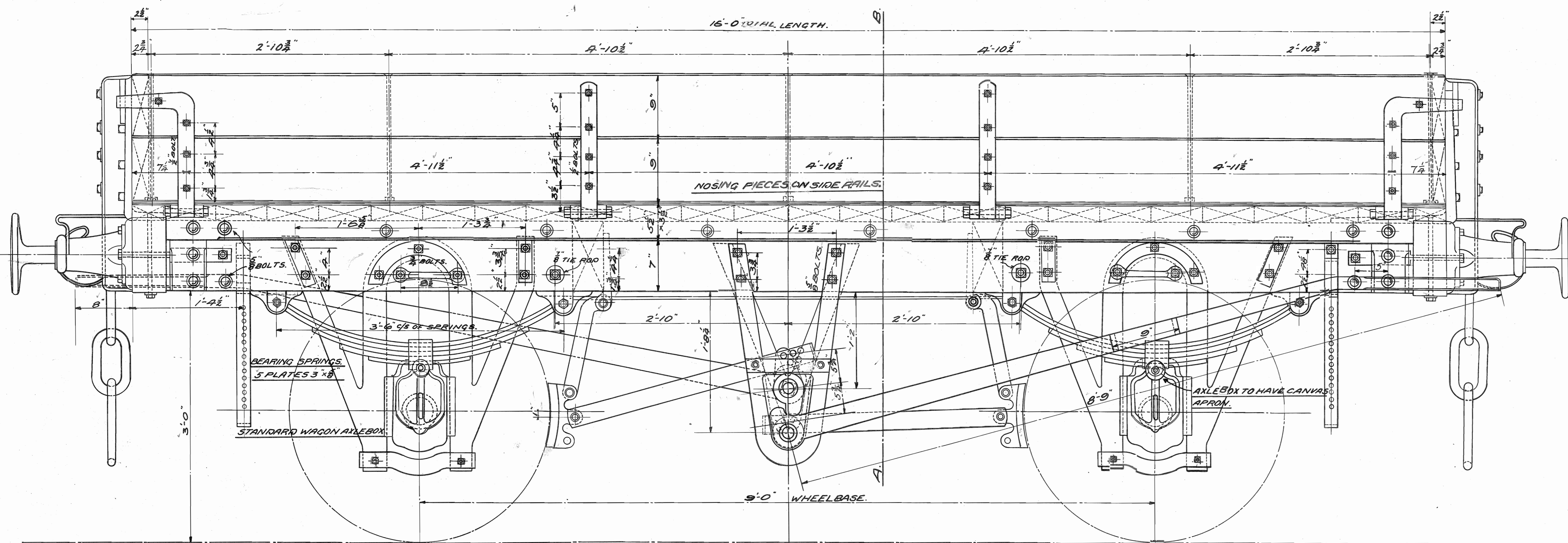
SIDE ELEVATION.
