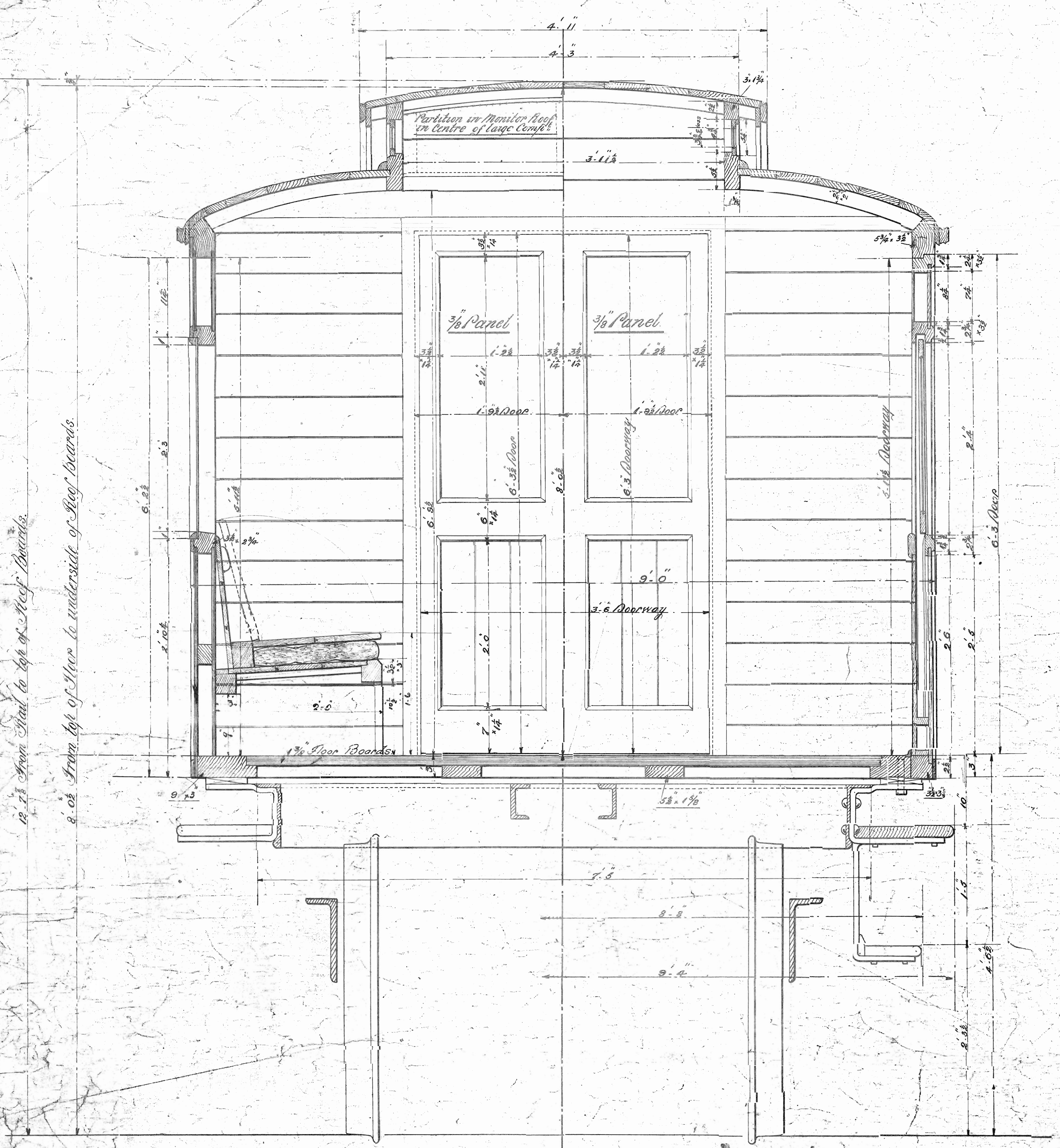
Half Cross Section thro' Comp. — Half Cross Section thro' Motor Comp.
