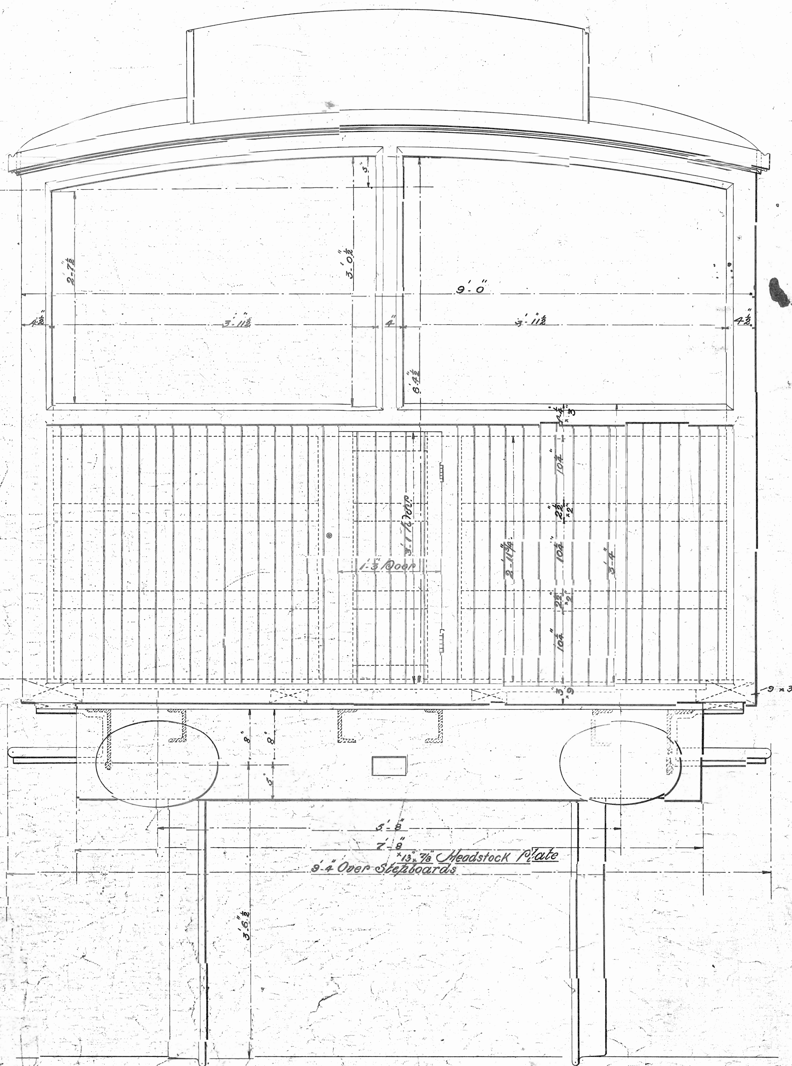
End Elevation.
