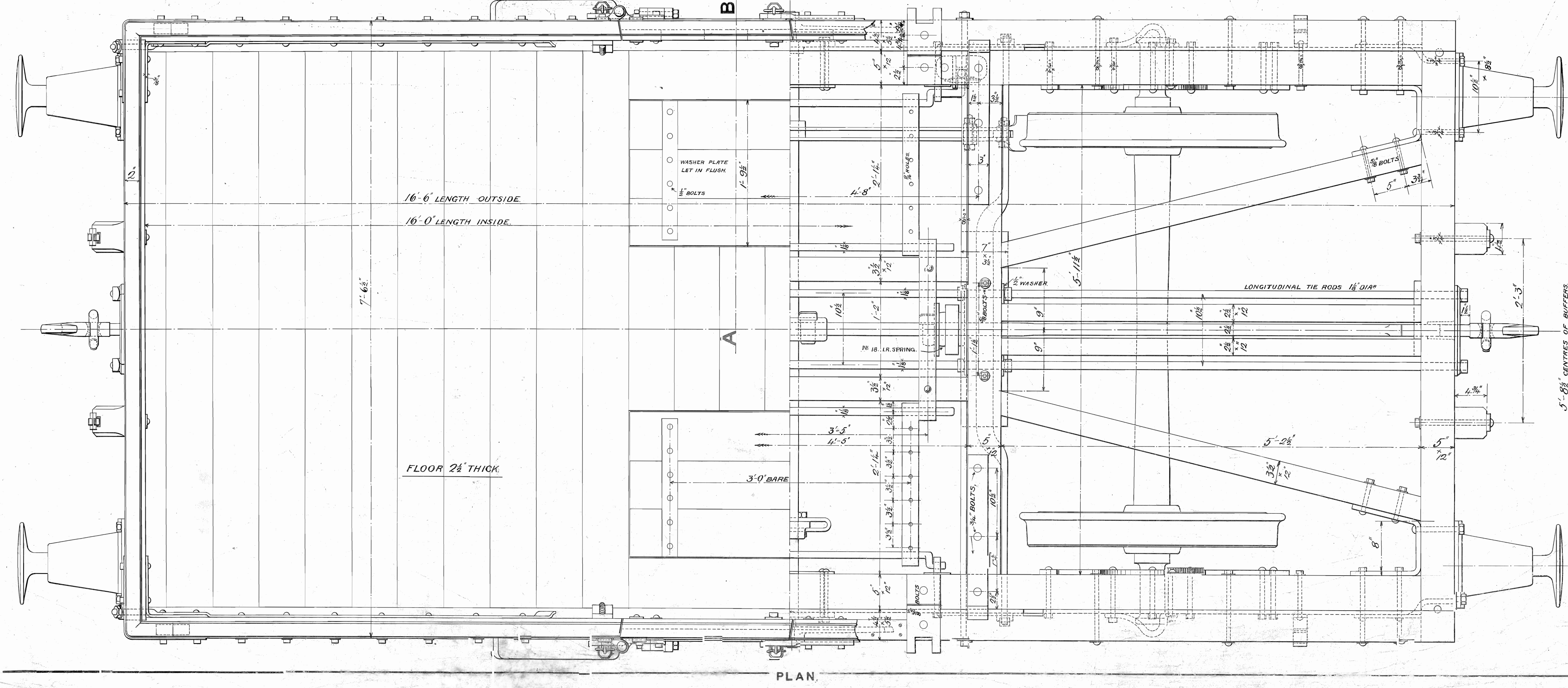
PLAN
