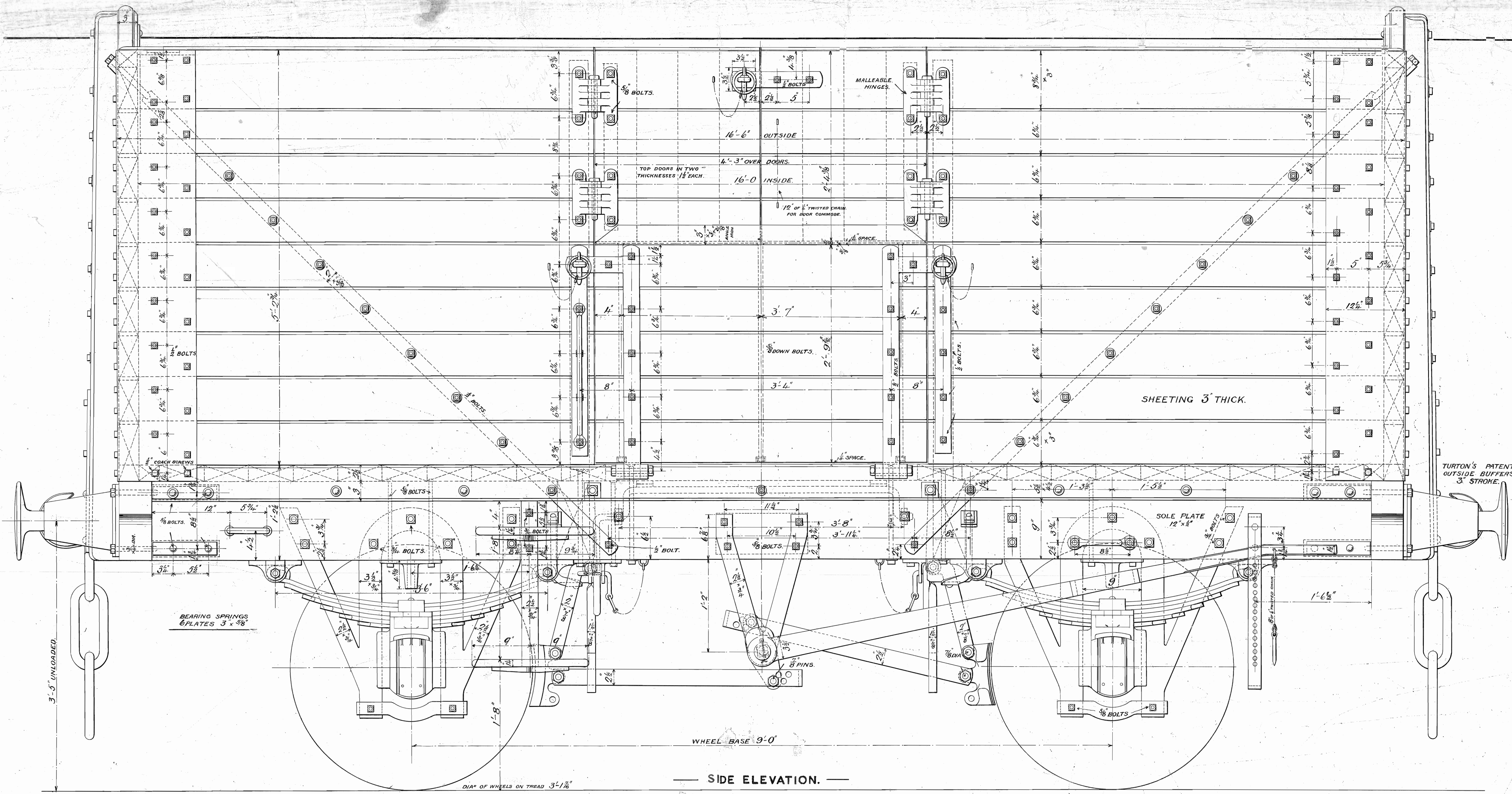
— SIDE ELEVATION. —
