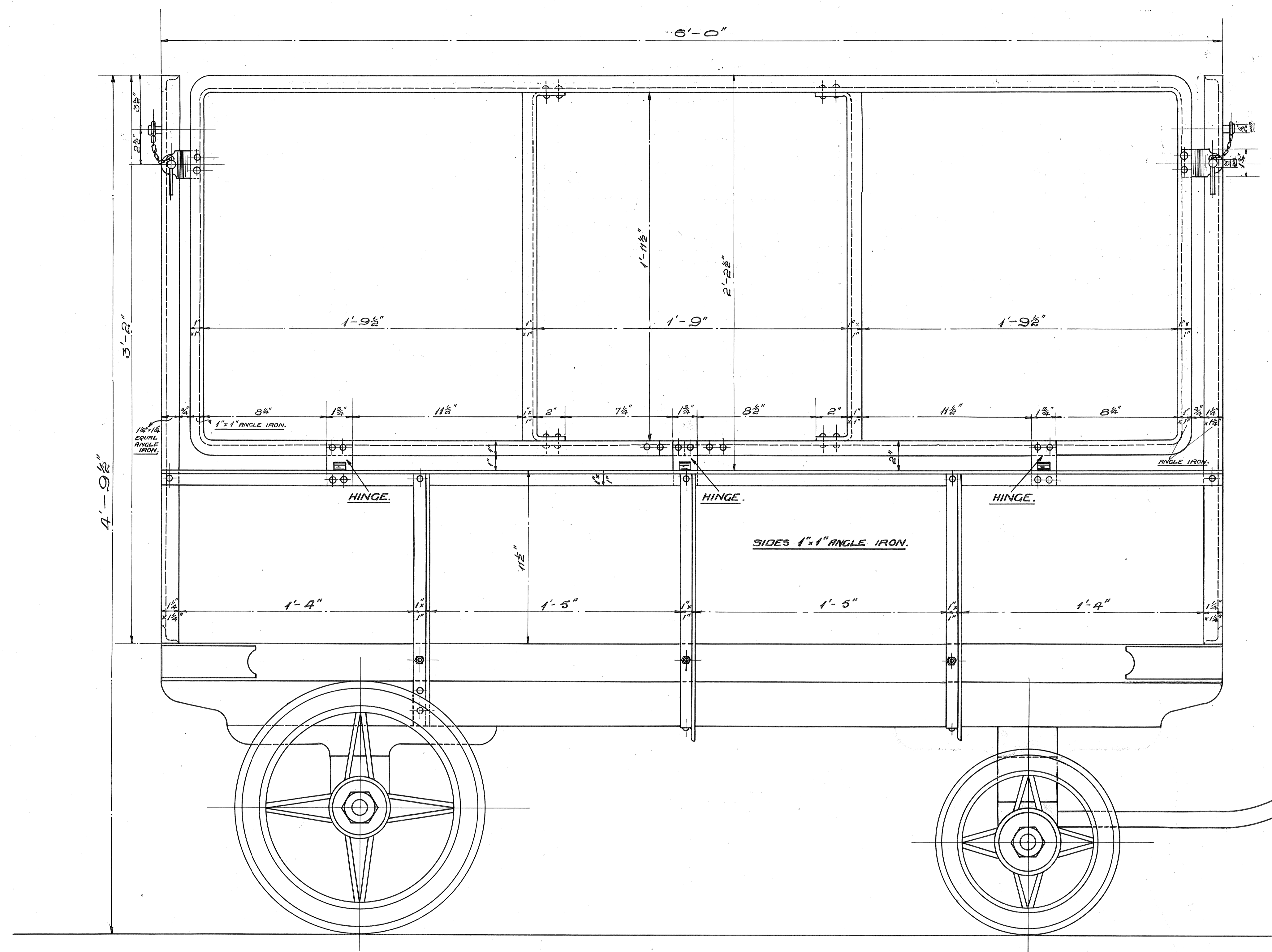
SIDE ELEVATION.
