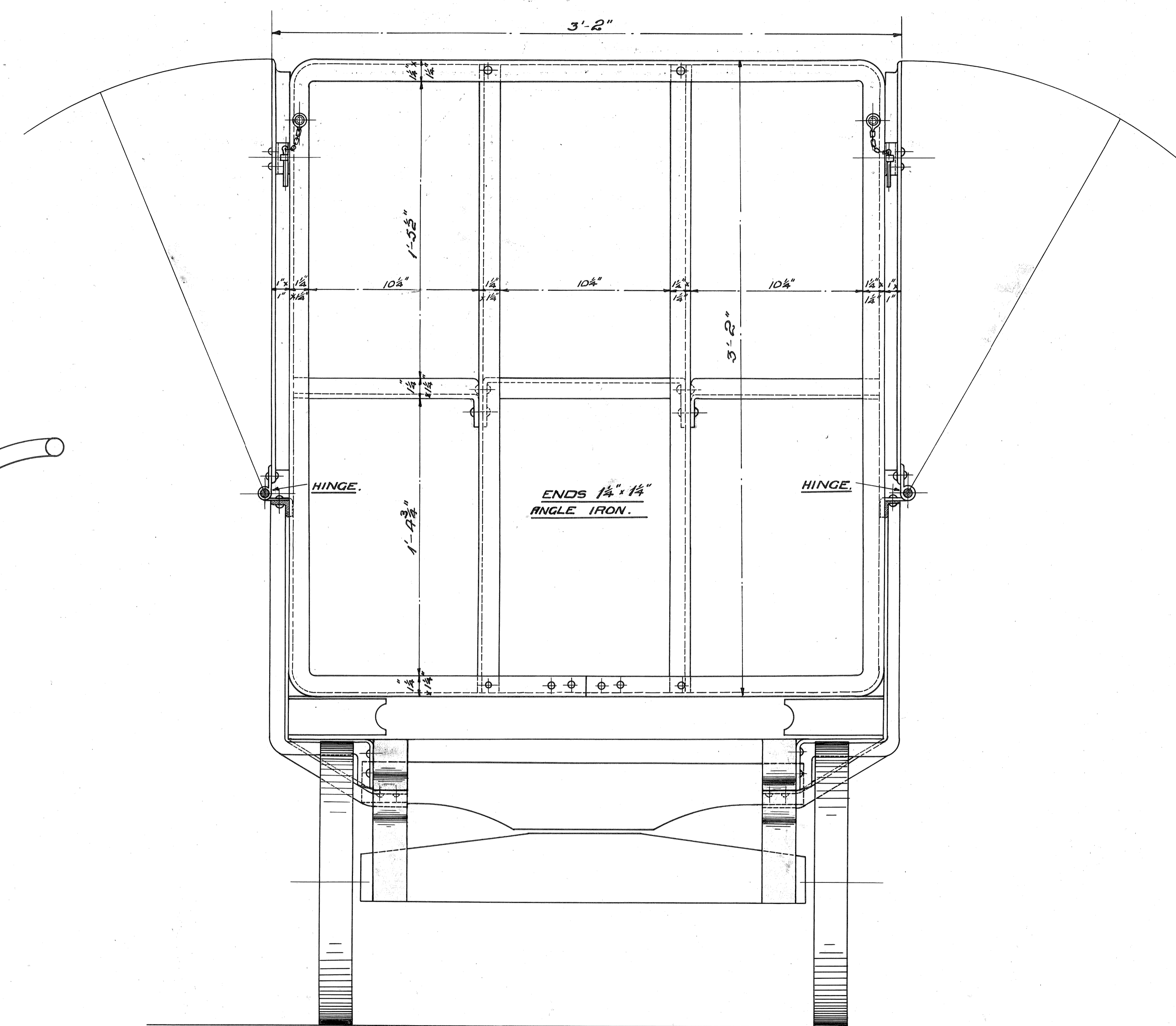
END ELEVATION.
